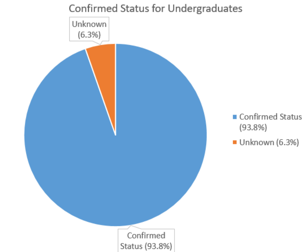
Chart 1: Confirmed Status
