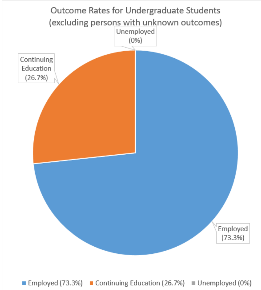
Chart 2: Outcome Rate
